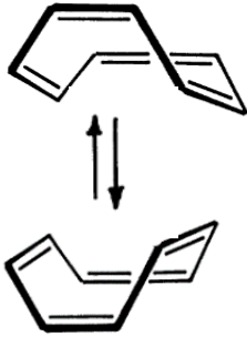
Ringinversion COT
